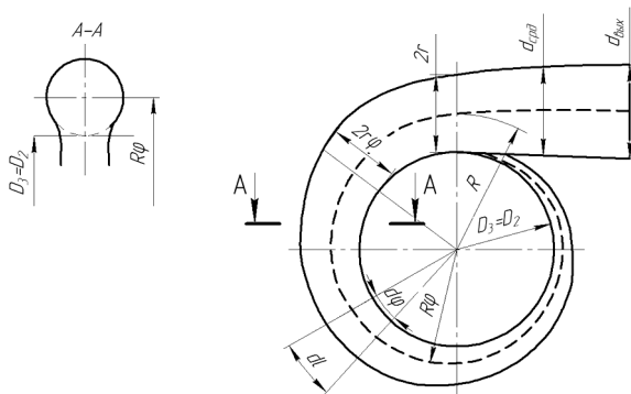
Fig. 9. Scheme for calculating losses in the spiral bend
