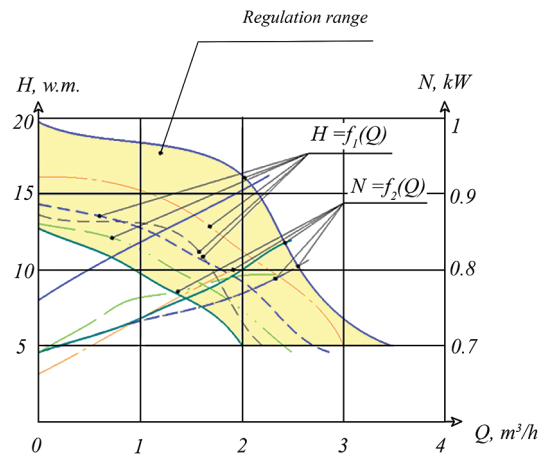
Fig. 5. Pressure-flow H = f_1(Q) and power N = f_2(Q) characteristics of a centrifugal pump with coaxial impellers:
