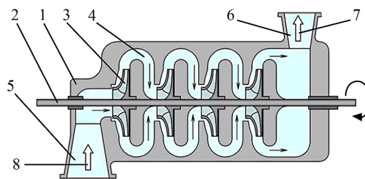
Fig. 1. Scheme of flow movement in a 4-stage centrifugal pump with channel outlets:
