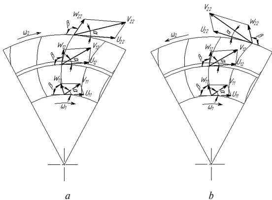
Fig. 8. Plan of speeds of impellers of a centrifugal pump with coaxial arrangement of impellers, depending on the direction of their rotation:
