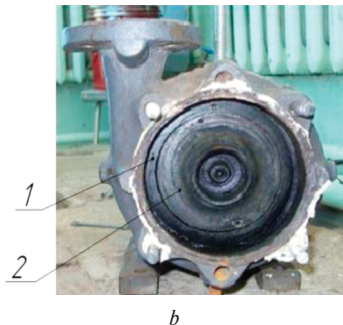
Fig. 4. Design of a centrifugal pump with coaxial impeller arrangement: 1 – external impeller; 2 – internal impeller
