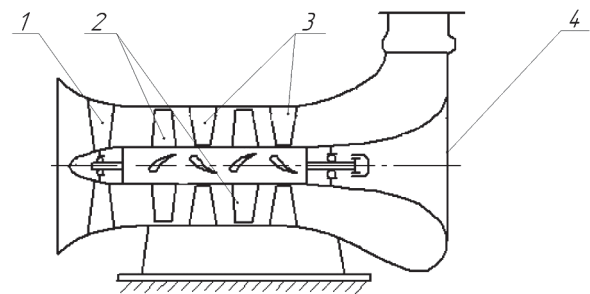
Fig. 7. Diagram of a two-stage axial blower: 1 – inlet guide vanes; 2 – impellers; 3 – straightening devices; 4 – blower housing
