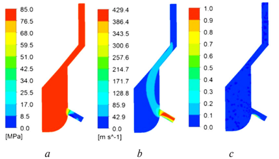
Fig. 5. Results of numerical simulation of mixed fuel (85 % of diesel fuel and 15 % of alcohol) flow in the injector nozzle flow path: a – fuel pressure distribution; b – flow rate distribution; c – vapour phase volume fraction distribution
